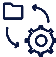
Data Processing
