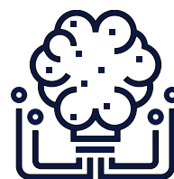
Machine Learning
