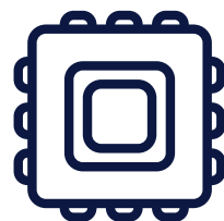
IOT Core
