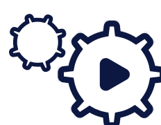
AI Engine
